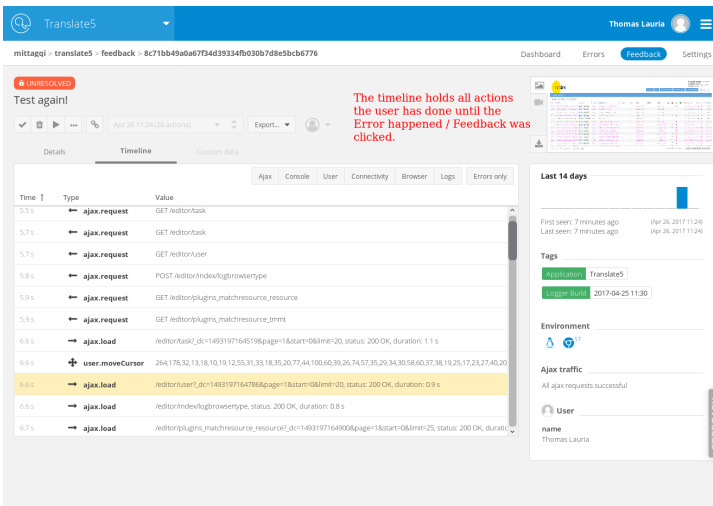
Illustration 2: List of actions taken by a user
